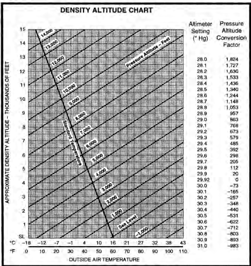
FIGURE 8—Density Altitude Chart.
